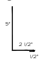
(10a) SIDEWALL
