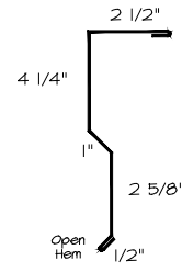
(10a) SIDEWALL
