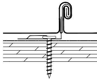
180° SEAM
